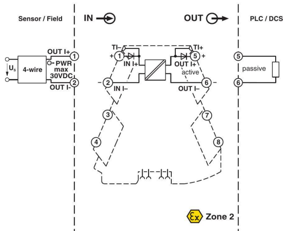
Figure 3 Block diagram
