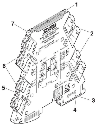
Figure 2 Structure
