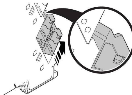
Figure 9 Disconnect position
