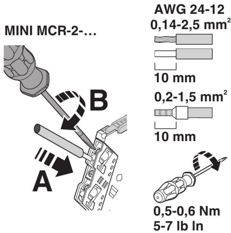
Figure 6 Screw connection
