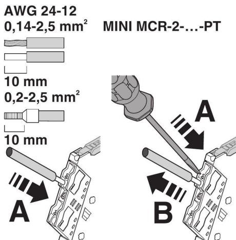
Figure 7 Push-in connection
