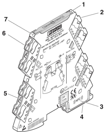
Figure 1 Structure
